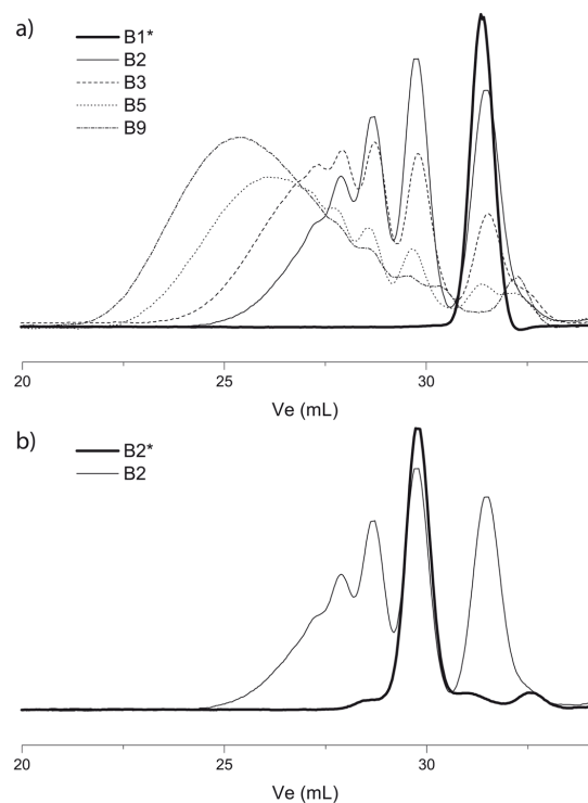
Fig. 2 SEC traces for oligomers (a) and dimer B2* (b).
