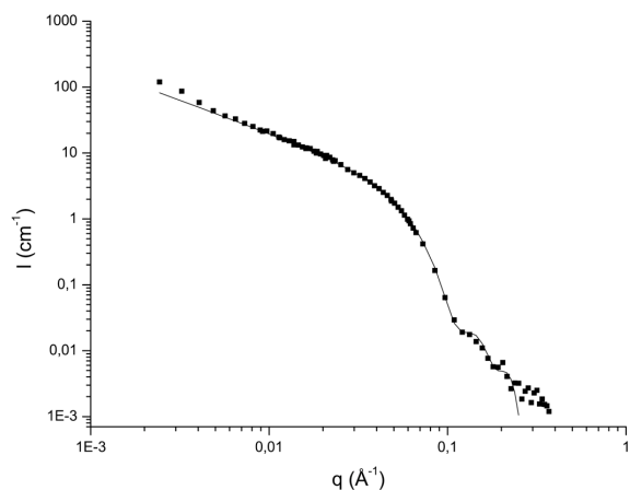
Fig. 6 SANS intensity ( I ) versus scattering vector ( q ) for monomer B1* solution in D 2 O at 10g/L and 25°C. The plain curve is a fit according to a model for two populations of long rigid filaments with a circular cross-section (respective cross-section diameters: 5.6 and 7.5 nm).
