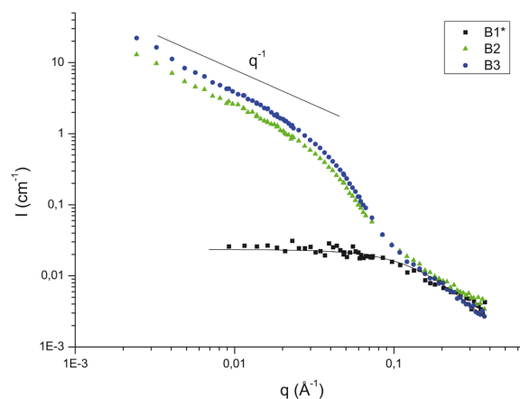
Fig. 7 SANS intensity ( I ) versus scattering vector ( q ) for monomer B1* and oligomers B2 and B3 solutions in CD 3 OD at 10g/L and 25°C.
