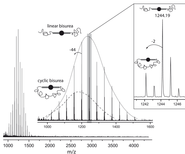
Fig. 3 MALDI-TOF spectrum for oligomer B3 .
