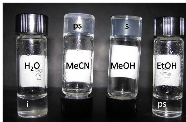
35 Fig. 4 Solubility tests for solutions of oligomer B2 (1%).
