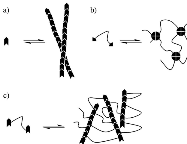
60 Fig. 1 Schematic assemblies formed by some amphiphiles: low molar mass compounds incorporating hydrogen bonds within a single hydrophobic group (a); polymers bearing multiple hydrophobic groups (b); polymers bearing multiple hydrophobic groups incorporating hydrogen bonds (c).
