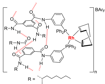
Figure 2. Proposed structure for the precatalyst derived from {}^H\text{BTA}^{\text{PPh}_2}(\text{S}),(\text{S}) . n , the degree of polymerization, depends on the reaction conditions; it is probably high in hexane, giving rise to a selective catalyst and low in \text{CH}_2\text{Cl}_2 (non-selective catalyst).
