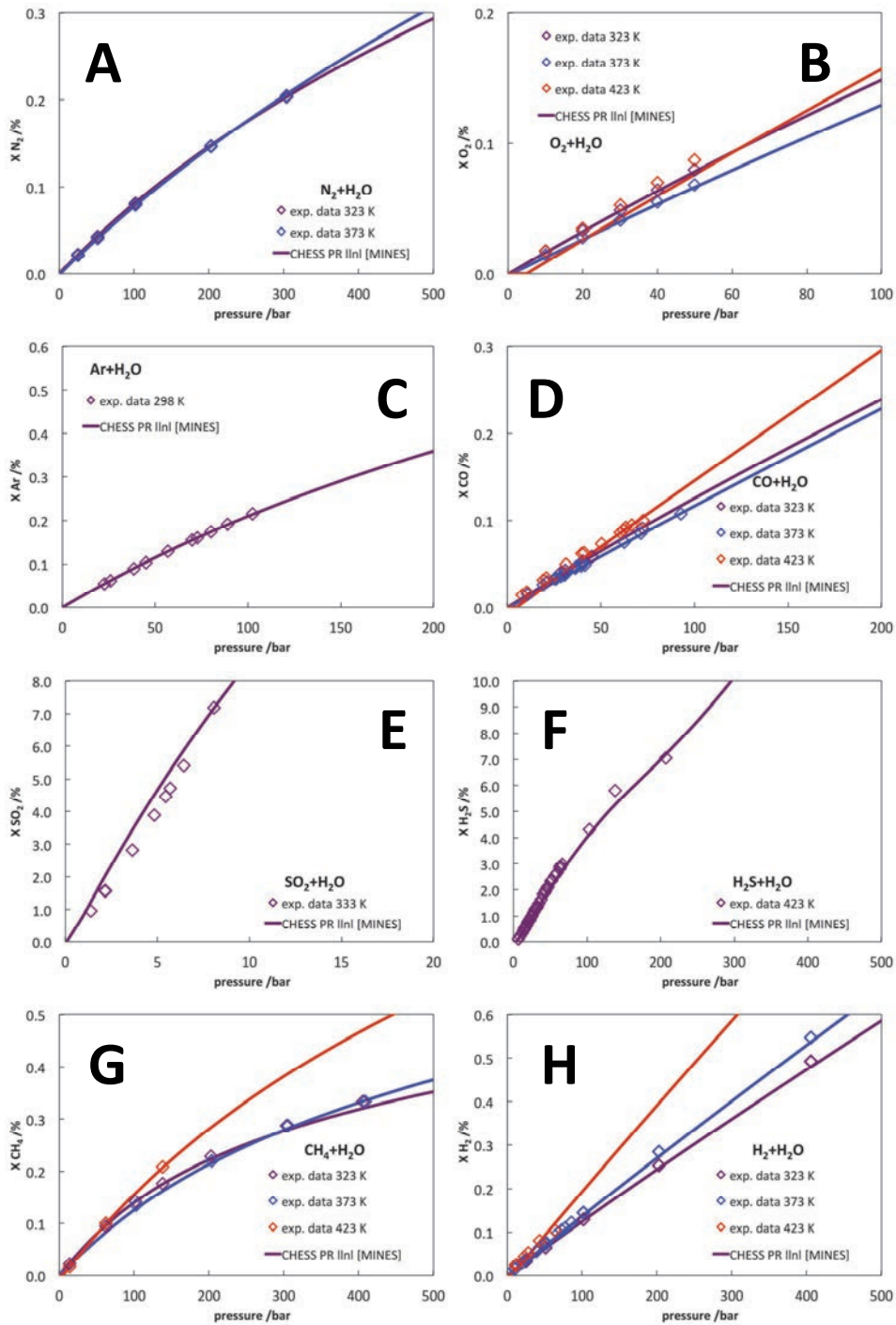
Fig. 2. Aqueous molar fraction (A) N_2 , (B) O_2 , (C) Ar, (D) CO, (E) SO_2 , (F) H_2S , (G) CH_4 and (H) H_2 vs. pressure for various gas+water systems and various temperatures. Symbols correspond to experimental measurements from the literature [25-33] and bold solid lines to CHES PR IlnI simulations.
