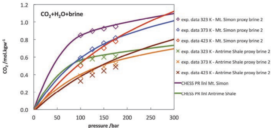
Fig. 6. Aqueous molality of CO 2 at at 323, 373 and 423 K, 150 bar in two synthetic proxy brine vs. pressure. Symbols correspond to experimental data [37] and bold solid lines to CHES simulations.
