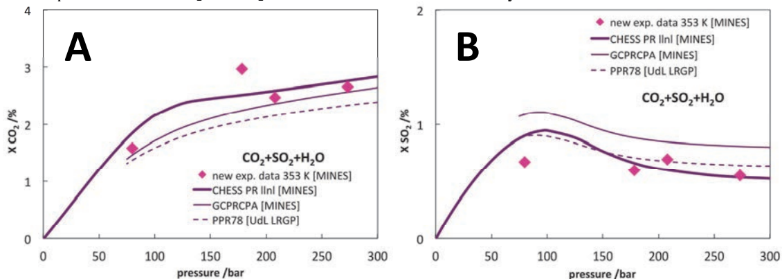
Fig. 3. Aqueous molar fraction (A) CO 2 and (B) SO 2 vs. pressure for CO 2 -SO 2 -H 2 O system (95% CO 2 and 5% SO 2 ) at 353 K. Symbols correspond to new measurements, thin solid lines to GC-PR-CPA model, thin dotted lines to PPR78 model and bold solid lines to CHES simulations.
