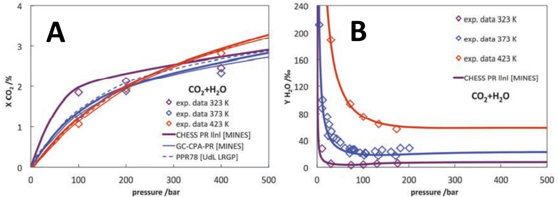
Fig. 1. Aqueous molar fraction (A) CO 2 and (B) H 2 O vs. pressure for CO 2 +H 2 O system at various temperatures. Symbols correspond to experimental measurements [3,23,24], thin solid lines to GC-PR-CPA model, thin dotted lines to E-PPR78 model and bold solid lines to CHESS simulations.
