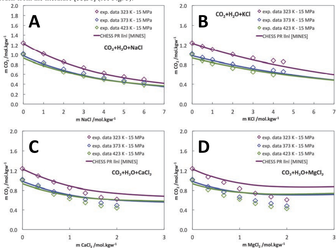
Fig. 5. Aqueous molality of CO 2 at 323, 373 and 423 K, 150 bar in (A) NaCl, (B) KCl, (C) CaCl 2 and (D) MgCl 2 vs. salt concentrations. Symbols correspond to experimental data [35,36] and bold solid lines to CHES simulations.
