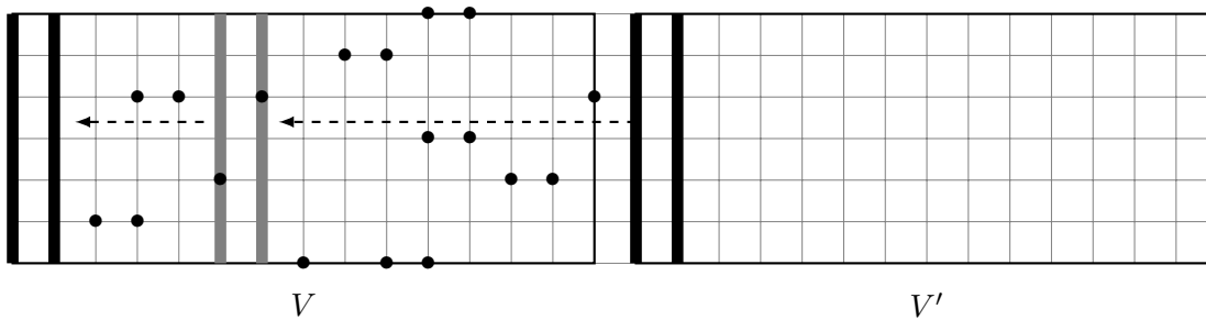
FIGURE 3. A sketch of the canonical path \Gamma_{\omega, \omega'} appearing in Lemma 3.8 for two horizontally adjacent blocks. Only the 1 st and 2 nd empty columns of the right super-good block are drawn (black). The black dots in the left block denote the empty sites, while the gray columns denote the different positions of the pair of adjacent columns inside the path. Notice the pair of adjacent empty sites on each row.
