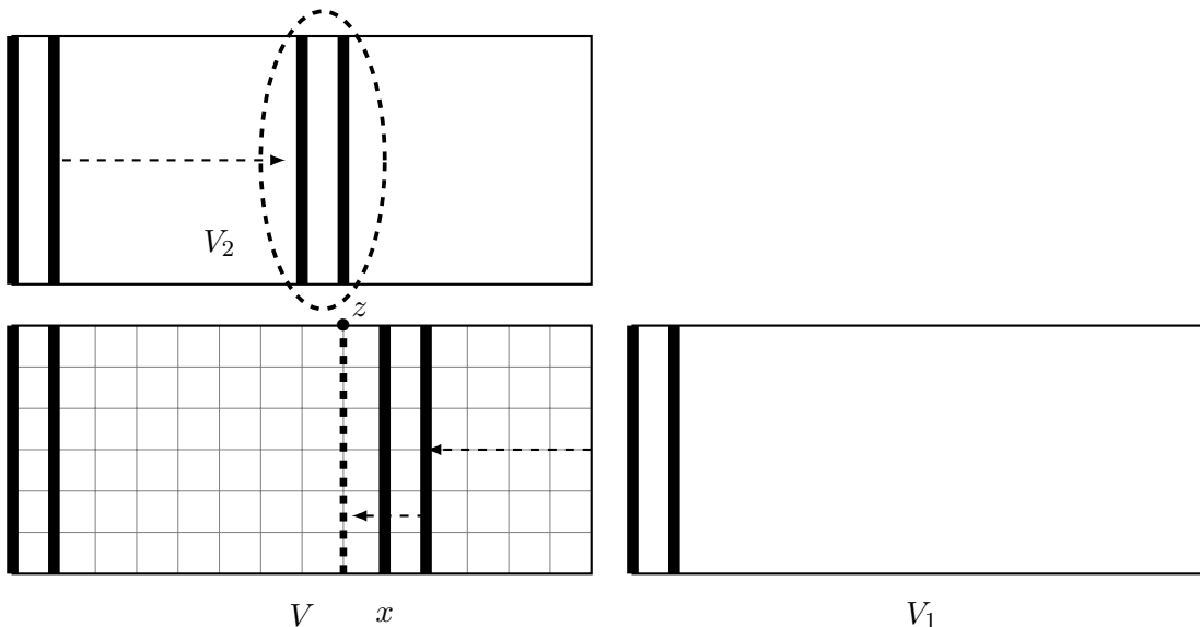
FIGURE 5. A sketch of the canonical path \Gamma_{\omega, \omega'} appearing in Lemma 3.7. Assuming that the path has been able to empty the two black columns of V , then it is possible to move these two columns one step further to the left as follows. First move the initial pair of double empty columns in V_2 to the new position encircled by the dashed ellipse, then, starting with the vertex z , empty the dashed black column in V and finally restore the original values of \omega to the right of x and then in V_2 .
