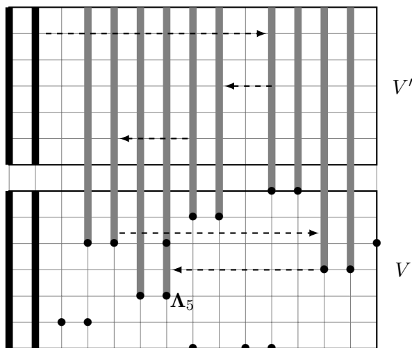
FIGURE 4. A sketch of the canonical path \Gamma_{\omega, \omega'} for two vertically adjacent blocks. The sequence of the dashed arrows must be read from top to bottom. Initially the 1 st and 2 nd empty columns of the top block (drawn in thick black) travel until they sit above the first pair of adjacent empty sites on the top row of the bottom block. At this time their height grows by one unit. Later in the path this new pair of empty columns is moved above the first pair of adjacent empty sites on the next to top row of the bottom block and so forth until the 1 st and 2 nd columns of the bottom block become empty.
