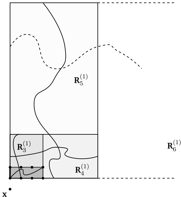
FIGURE 2. A drawing of the first five rectangles \{R_n^{(1)} + x\}_{n=1}^5 together with a pictorial representation of the hard crossings of zeros (the solid lines) required by the auxiliary constraint c_x^{(n,1)} . The dashed curved line represents a piece of the hard crossing for the next rectangle R_6^{(1)} + x (the two horizontal dashed lines). Notice that each rectangle has its leftmost lowermost vertex always at x + \vec{e}_2 and that the first rectangle R_1^{(1)} consists of only two vertices, x + \vec{e}_2 and x + 2\vec{e}_2 .
