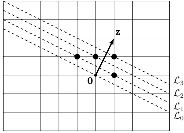
FIGURE 1. An example in two dimensions of a constraint satisfying the exterior condition w.r.t. a sequence of increasing half-spaces. Only the slices \{\mathcal{L}_n\}_{n=0}^3 are drawn. The constraint c_0 requires that the restriction of the configuration \omega to each one of the four vertices around the origin (black dots) belongs to a certain subset G \subset S .
