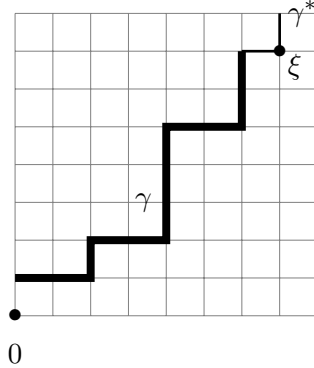
FIGURE 1. The minimal good path \gamma^* , the position of the first super-good vertex \xi encountered while traveling backward along \gamma^* , and the subpath \gamma \subset \gamma^* (thick black) connecting \vec{e}_2 to a neighbour of \xi .
