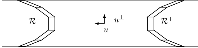
FIGURE 7. The two quasi-stable half-rings \mathcal{R}^\pm . For simplicity they have been drawn as specular to each other although in general \mathcal{Q}(-C) \neq -\mathcal{Q}(C) .
