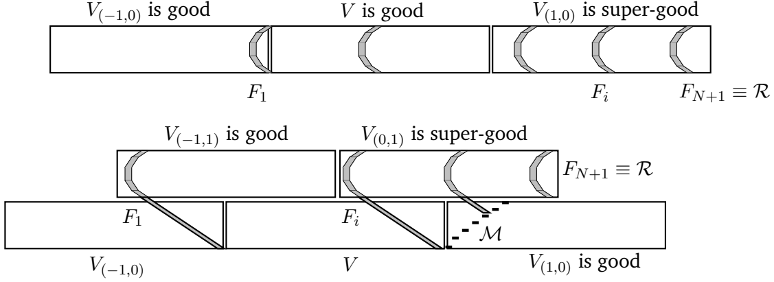
FIGURE 6. A sketchy picture illustrating the local neighborhood W_1 (above) and W_2 (below) of the block V = V_{(0,0)} , together with their structure of the good and super-good blocks. For I_1 (above) the fibers are simply the disjoint translates of the rightmost empty half-ring \mathcal{R} in the last quarter of V_{(1,0)} . For I_2 (below) the fibers are not all equal and they change at the steps of the increasing stair \mathcal{M} (the little horizontal intervals). Each fiber then becomes an elongated version of the rightmost empty half-ring \mathcal{R} .
