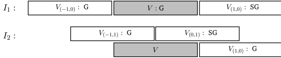
FIGURE 5. For simplicity we fix i = (0, 0) . In I_1 the box V \equiv V_{(0,0)} is conditioned to be good (G) while the boxes V_{(-1,0)} and V_{(1,0)} are good and super-good (SG) respectively. The set \mathbb{L}^+((0, 0)) appearing in I_2 consists of the two boxes V_{(1,0)} and V_{(-1,1)} . These boxes are good, the box V_{(0,1)} is super-good while V is unconditioned.
