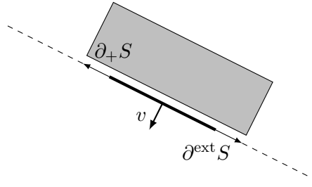
FIGURE 3. The + -boundary of S , the external boundary (solid segment) and its subset \partial_\lambda^{\text{ext}} S (thick solid segment)
