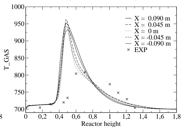
Figure 6. WD_700_MESH1 : numerical against experimental mean gas temperature (°C)
