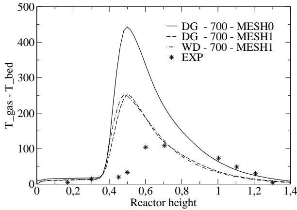
Figure 7. All simulations: numerical against experimental mean gas temperature ( ^{\circ}\text{C} )
