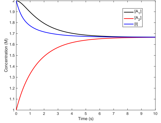
Fig. 1. Time evolution of the concentrations governed by (9) with [A_1](0) = 2 M , [A_2](0) = 1 M , [I](0) = 2 M and k_{A,1} = 1 s^{-1} , k_{A,2} = 0.5 s^{-1} , k_{I,1} = 1 s^{-1} , k_{I,2} = 0.5 s^{-1} .
