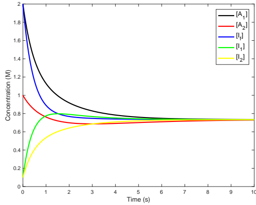
Fig. 4. Time evolution of the concentrations governed by (18 with [A_1](0) = 2 M , [A_2](0) = 1 M , [I_f](0) = 2 M , [I_1](0) = 0.1 M , [I_2](0) = 0.1 M and k_{A,1} = 1 s^{-1} , k_{A,2} = 0.5 s^{-1} , k_{I_1} = 1 s^{-1} , k_{I_2} = 0.5 s^{-1} , k_{I_1,f} = 1 s^{-1} , k_{I_2,f} = 0.5 s^{-1} .
