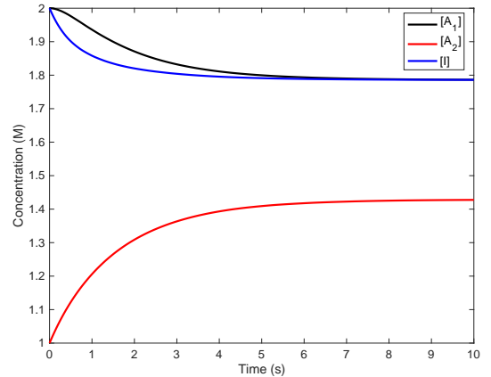
Fig. 2. Time evolution of the concentrations governed by (9) with [A_1](0) = 2 M , [A_2](0) = 1 M , [I](0) = 2 M and k_{A,1} = 1 s^{-1} , k_{A,2} = 0.5 s^{-1} , k_{I,1} = 1 s^{-1} , k_{I,2} = 0.4 s^{-1} .
