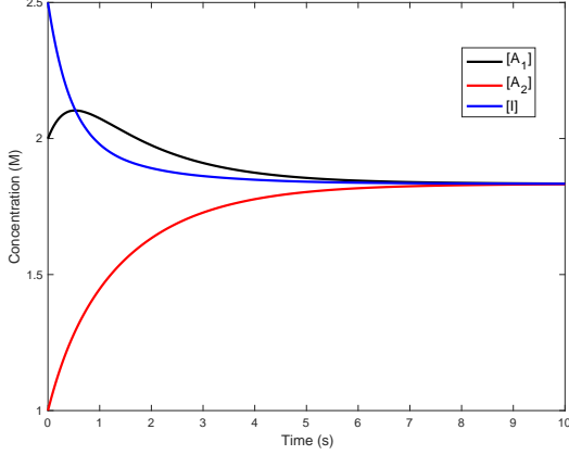
Fig. 3. Time evolution of the concentrations governed by (9) with [A_1](0) = 2 M, [A_2](0) = 1 M, [I](0) = 2.5 M and k_{A,1} = 1 s^{-1}, k_{A,2} = 0.5 s^{-1}, k_{I,1} = 1 s^{-1}, k_{I,2} = 0.5 s^{-1} .
