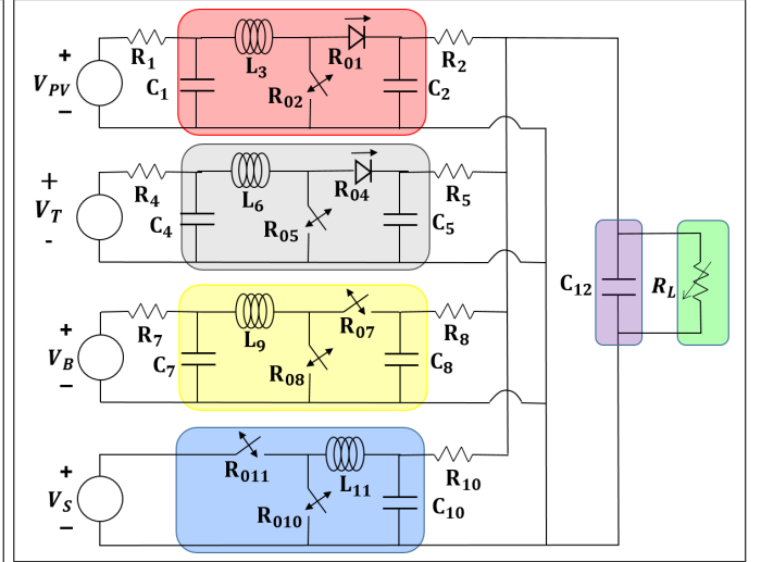
Figure 2: The considered framework: A circuit scheme.
