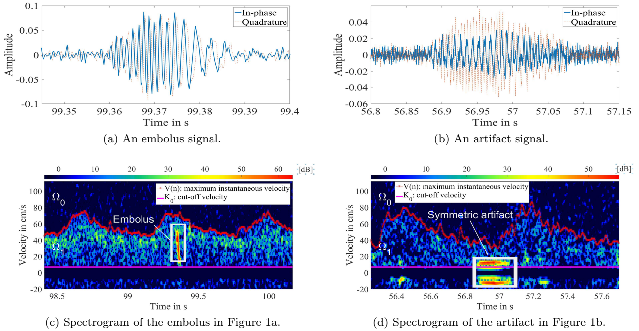
Fig. 1: Example of HITS representations.
