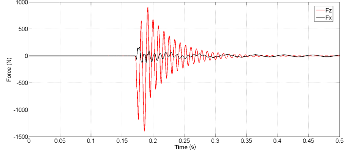
Figure 6: Vertical force and longitudinal force at the wheel center during dynamic contact on a 5 x 10 mm bar for the circular ring.
