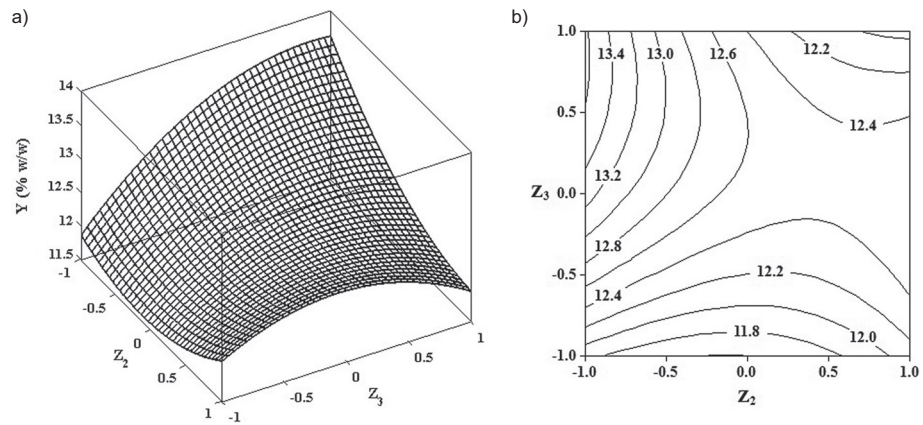
Figure 6 Response surface a) and contour b) plots for the effect of scrubbing solution temperature and liquid-to-gas volumetric ratio on Y at initial NaOH concentration of 20% w/w.
