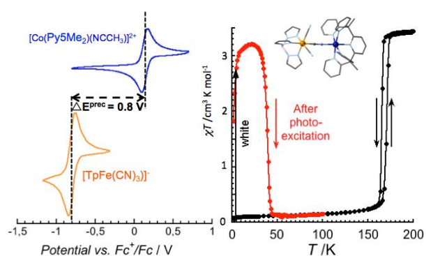
Figure 6 (left) Cyclic voltammety of the two precursors [\text{Co}(\text{Py5Me}_2)(\text{NCCH}_3)]^{2+} and [\text{TpFe}(\text{CN})_3]^- used for the synthesis of the pair 6 (right) Plot of \chi T vs temperature for the pair \{[(\text{Tp})\text{Fe}(\text{CN})_3][\text{Co}(\text{Py5Me}_2)(\text{OTf})]\} 6 in the dark (black points, 0.4 K/min) and after white light irradiation at 10 K.
