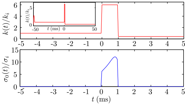
FIG. 1: The two signals \tilde{k}(t) and \sigma_o(t) used to drive fast expansion. The time is set to zero when the decompression is triggered. The inset exhibits the full dynamics used in the experiment, cycled 4 \cdot 10^4 times. The system is initialized at t = -50 ms with an ESE-compression from \tilde{k}_f to \tilde{k}_i , (noiseless TESE with Eqs. (4) and (5)), then left unperturbed, before the decompressing-TESE is applied at t = 0 . The system is subsequently left unperturbed up to t = 50 ms, before the cycle repeats. The TESE sector ( 0 \leq t \leq t_f = 1 ms) is ruled by Eqs. (5), (8) and (9). Here, \tau_f = 11 ms, \tau_i/\tau_r = 100 , \chi \equiv k_f/k_i = 0.44 and k_{\max} = 6 .
