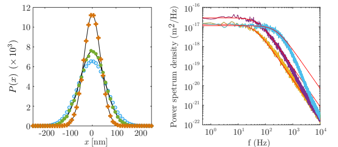
FIG. 2: (a) Density P(x, t) measured in the initial compressed state (orange crosses), and at the end of the protocol at t = t_f (green dots). The measured pdf are in excellent agreement with the target densities shown with lines, for a decompression factor \chi = 0.44 . We also measure the stationary pdf when the random force is switched on (blue circles, for a higher stiffness k = 4k_i ). (b) Power spectra of x measured in equilibrium at k = k_i without (orange line) and with noise (purple line). In this case, \sigma_i = 30 nm, f_c = 41 Hz and \sigma_o = 20 nm. We also show a power spectrum for k = 4k_i with noise ( \sigma_o = 21 nm, blue line) corresponding to the blue circles in (a). The Lorentzian fits allow us to calibrate the system and the noise amplitude. Beyond the filtering frequency f_{\text{lp}} = 1 kHz, the fits become meaningless and all curves eventually collapse.
