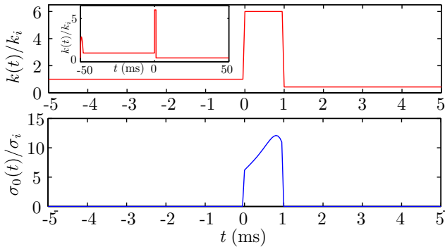
FIG. 1: The two signals \tilde{k}(t) and \sigma_o(t) used to drive fast expansion. The time is set to zero when the decompression is triggered. The inset exhibits the full dynamics used in the experiment, cycled 4 \cdot 10^4 times. The system is initialized at t = -50 ms with an ESE-compression from \tilde{k}_f to \tilde{k}_i , (noiseless TESE with Eqs. (4) and (5)), then left unperturbed, before the decompressing-TESE is applied at t = 0 . The system is subsequently left unperturbed up to t = 50 ms, before the cycle repeats. The TESE sector ( 0 \leq t \leq t_f = 1 ms) is ruled by Eqs. (5), (8) and (9). Here, \tau_f = 11 ms, \tau_i/\tau_r = 100 , \chi \equiv k_f/k_i = 0.44 and k_{\max} = 6 .
