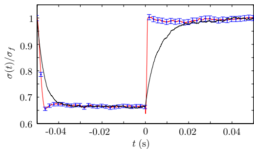
FIG. 3: Dynamics of the standard deviation \sigma(t) of the Brownian particle position, for two distinct cyclic schemes. The first one alternates between ESE for compression phases and TESE for decompression phases (red line), while the second one is only constituted of STEP procedures (black line). Time t = -50 ms corresponds to the beginning of the compression phase, where the stiffness is changed from k_f to k_i , and time t = 0 is the beginning of the expansion phase, where k is switched from k_i to k_f < k_i (see also Fig. 1). The experimental measures are shown, together with error bars. To gather relevant statistics, the scheme is repeated as explained in the main text and in Fig. 1.
