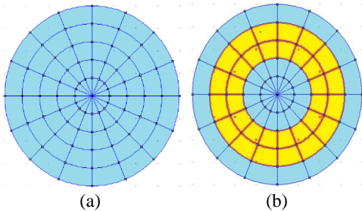
Fig.5. Inductor mesh in the plane (r, z) .
