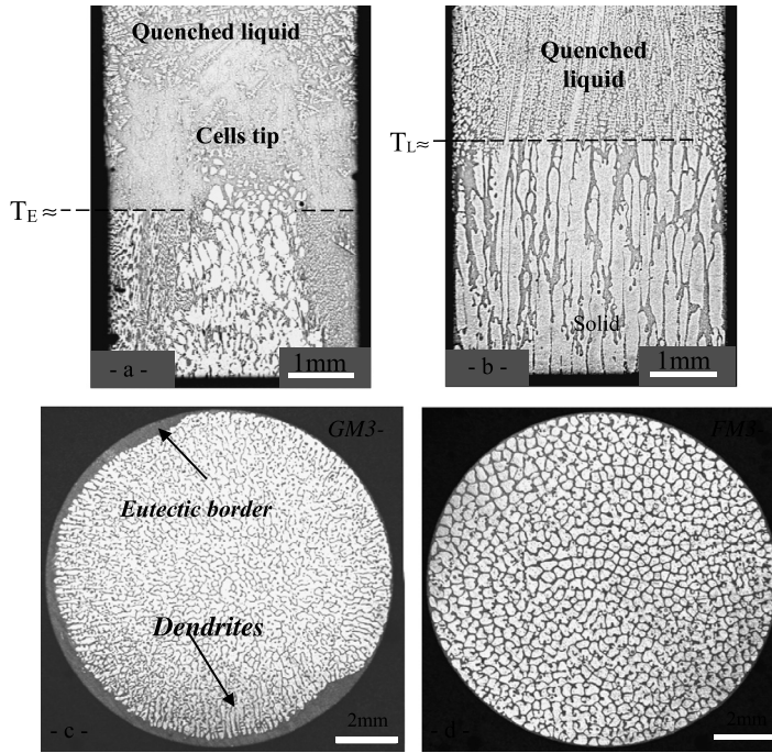
Fig. 6. Comparison of the microstructures obtained during upward solidification on ground (a and c) and in microgravity (b and d) for Al–1.5wt%Ni, G = 24 \text{ K/cm} and V = 2.3 \text{ }\mu\text{m/s} . (a) and (b): Longitudinal sections across the quenched front, (c) and (d) transverse sections below the quenched front.
