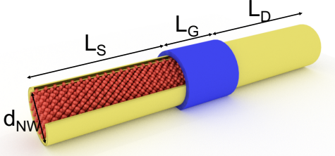
FIG. 1. (Color online) Schematic representation of the silicon GAA NW transistors considered in this work (with a \langle 100 \rangle crystallographic orientation in the present case). The length of the gate is L_G = 5 nm, the source and drain extensions L_{S/D} = 15 nm, and the diameter of NW d_{NW} = 3 nm. Source and drain regions are doped with a doping concentration of donors or acceptors N_{D/A} = 1 \times 10^{20} \text{ cm}^{-3} . Si \langle 110 \rangle , Si \langle 111 \rangle , and Ge \langle 110 \rangle are also considered (not shown).
