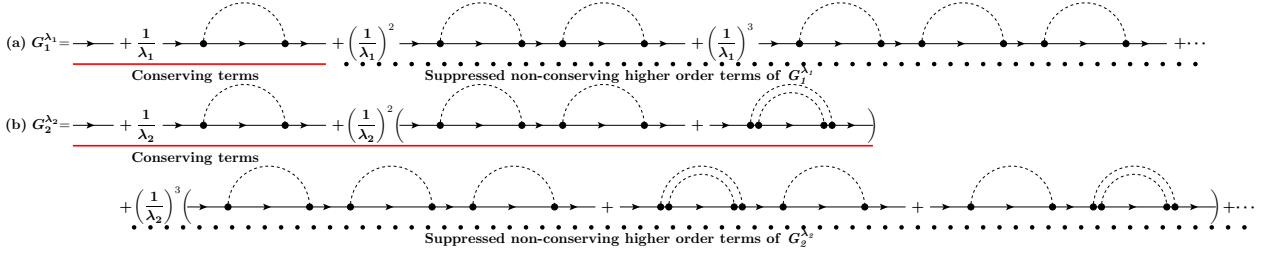
FIG. 2. (Color online) Rescaled Green's functions, (a) G_1^{\lambda_1} of first SCBA iteration and (b) G_2^{\lambda_2} of second SCBA iteration, described by Feynman diagrams. Conserving and non-conserving terms are arranged in ascending order in interaction. Thin lines with an arrow indicate electron non-interacting Green's function. Dashed lines are for free phonon propagators.
