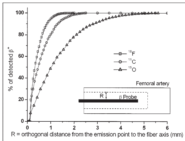
FIGURE 2. For ^{18}\text{F} -, ^{11}\text{C} -, and ^{15}\text{O} -labeled molecules, Monte Carlo evaluation of the fraction of detected signal corresponding to radioactivity in the femoral artery as a function of artery radius.
