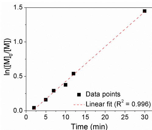
Figure 3. First order plot for the bulk copolymerization of VAc and MAF-TBE at 40 °C initiated by V-70 in the presence of 3 \{[\text{VAc}]_0 + [\text{MAF-TBE}]_0\}/[\text{V-70}]_0/[\mathbf{3}]_0 = 537/3/1 , [\text{VAc}]_0/[\text{MAF-TBE}]_0 = 1/1 .
