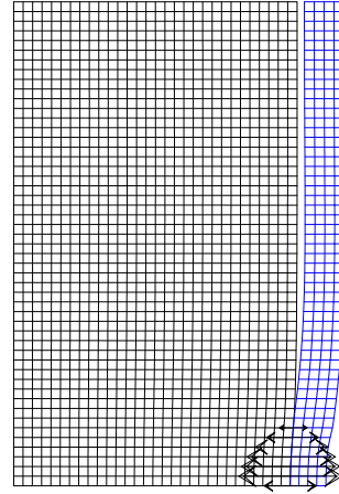
Figure 18: Frictionless 2D(r,z) test case: contact forces for h_0 = 200 \mu\text{m}
