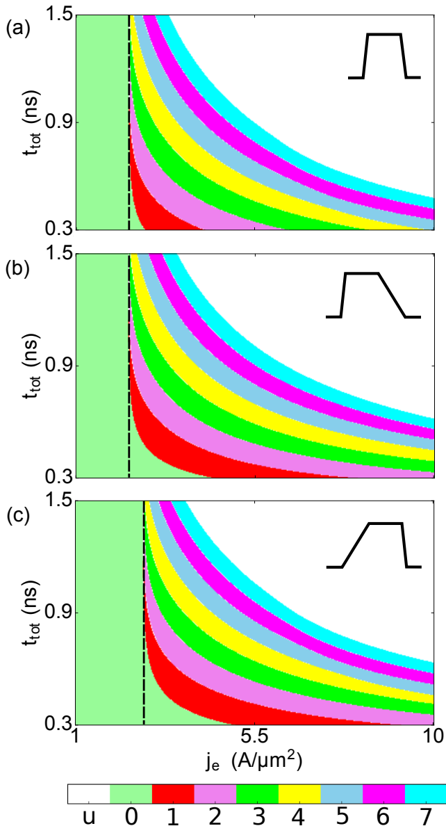
FIG. 3. (Color online) Influence of the pulse shape on the phase diagram for a DW at T=0\text{K} in an infinite nanostrip. The parameter space is the total time ( t_r + t_s + t_f ) vs. current amplitude. (a) Symmetric pulse with t_r = t_f = 5 ps and t_z = 10 ns, Asymmetric pulse with (b) t_r = 5 ps, t_f = 300 ps and t_z = 10 ns, and (c) t_r = 300 ps, t_f = 5 ps and t_z = 10 ns. The upper right region is due to the finite size of the simulated window.
