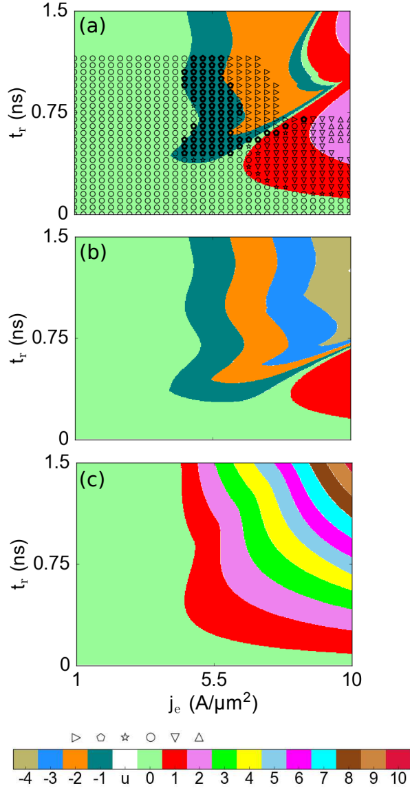
FIG. 6. (Color online) Influence of the pulse raise time t_r on the phase diagram for a DW at T=0\text{K} in an infinite nanostrip for different parameters \alpha and \beta . The parameter space is the raise time vs. current amplitude. In all cases, t_s = t_f = 5 ps and t_z = 10 ns. (a) \alpha = 0.02 and \beta = 0.04 , (b) \alpha = \beta = 0.02 , and (c) \alpha = 0.05 and \beta = 0.1 . In (a) the micromagnetic results (scattered symbols) are compared to the 1D model (colored regions), while in (b) and (c) only 1D model results are shown. At high currents, the micromagnetic results give several unintended states (the empty scattered symbol region to the right of (a)).
