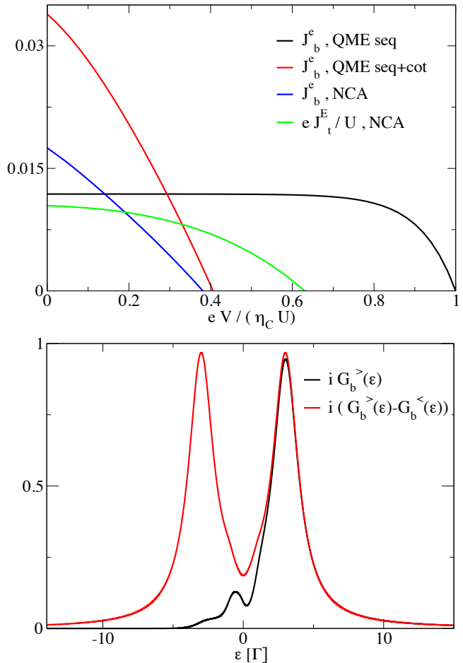
FIG. 3: Top panel: Charge current in e\Gamma/\hbar units, evaluated in the QME and in the NCA, for U = 6\Gamma , T_h = \Gamma , and T_c = 0.2T_h . The renormalized energy current evaluated in the NCA, \frac{eJ_t^E}{U} is also presented. Bottom: Green's functions for the same parameters, and for V equal to the upper panel stopping voltage.
