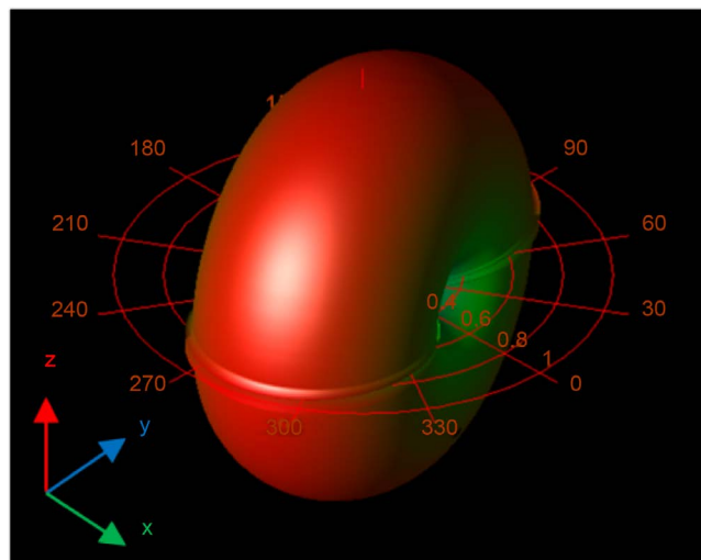
Figure 8. ISM antenna 3D normalized radiation pattern.
