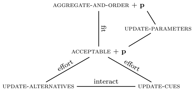
Fig. 12: Interdependence of function parameters.
