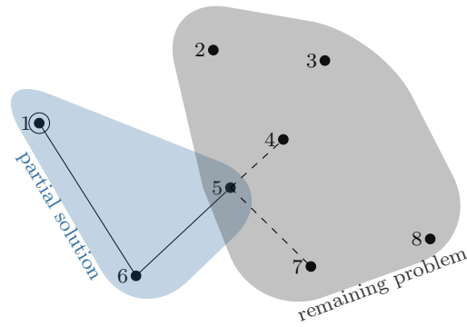
Fig. 3: Representation of TSP instances and states in the solution process. The numbers next to the points are labels. The partial solution starts at point 1 and includes points 6 and 5. Point 5 is the current point from which to decide the next step. Points 4 and 7 are alternatives for the next decision.
