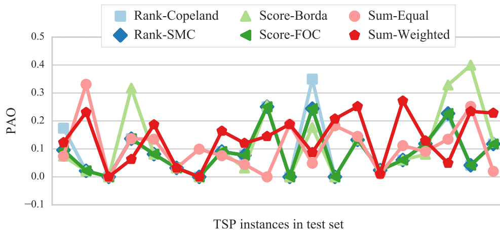
Fig. 5: (Unnormalized) PAO of optimized configurations for 20 test tasks.
