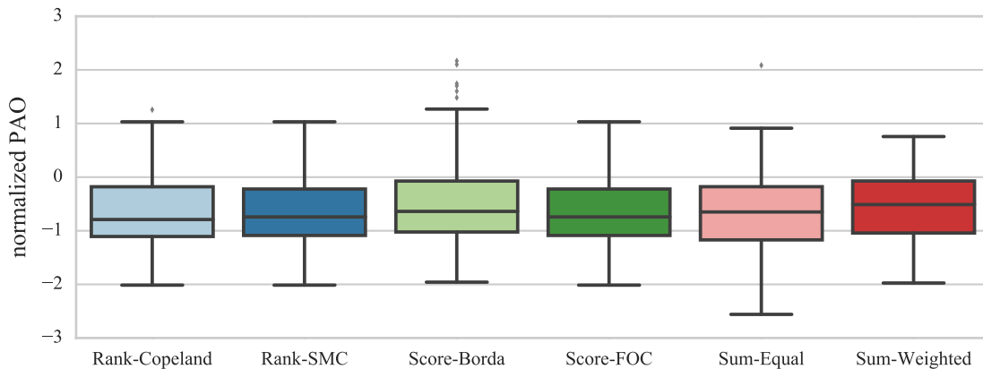
Fig. 4: Quality with optimized configurations over 70 test tasks. Lower values denote shorter, i.e. better, tours.
