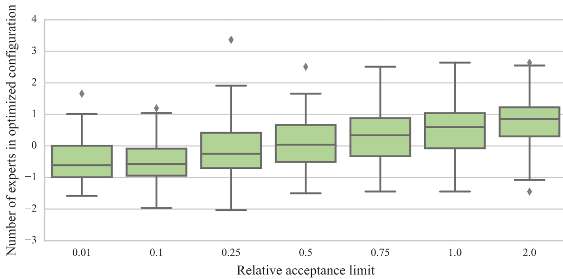
Fig. 9: Acceptance parameter \eta for ttb condition.
