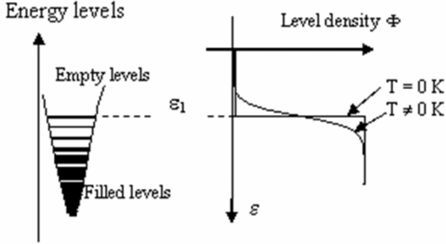
Fig. 3. Energy level distribution. At the temperature T = 0 K, the energy \varepsilon_1 is the border between the filled levels and the empty ones. Then the level density curve exhibits a step at \varepsilon_1 . If the temperature is T \neq 0 K, there are some filled levels above this energy.
