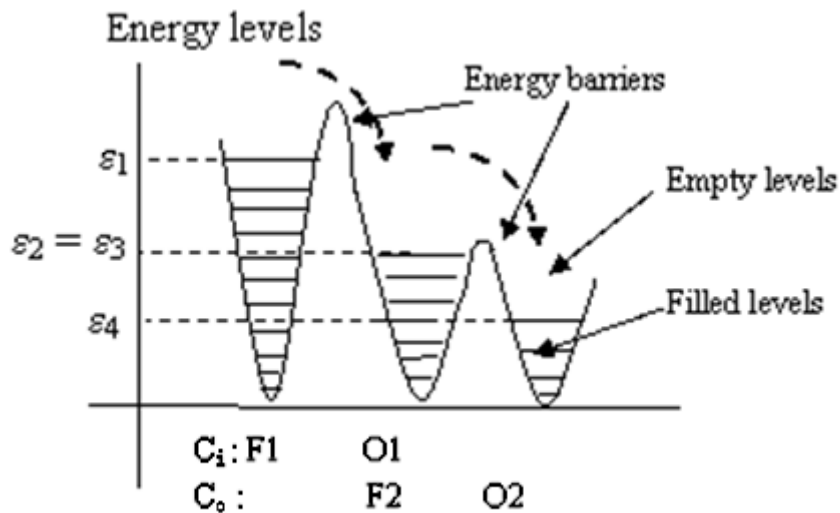
Fig. 2. Closed-open transitions. An energy \Delta\varepsilon arriving in a closed channel causes energy barrier decay. F1: energy levels of an equivalent charge of a closed inward channel C_i . O1: energy levels of an equivalent charge of an open inward channel C_i . F2: energy levels of an equivalent charge of a closed outward channel C_o . F2 is the same that O1. O2: energy levels of an equivalent charge of an open outward channel C_o .
