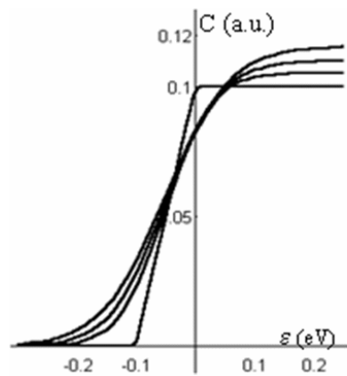
Fig. 7. Transmembrane energy dependence of conductance. T = 300 K.
