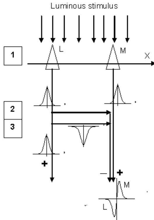
Fig. 1. Diagram model used to understand how a wavelet can be constructed. The direct pathways are constituted by the photoreceptors (M- and L-cone), the bipolar cells, and the ganglion cells. These pathways transmit the information without change (plus sign). The lateral pathways are constituted by the horizontal cells (2) and the amacrine cells (3). These pathways transmit the information with change in the sign (minus sign).
