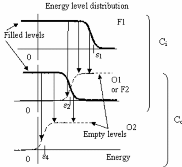
Fig. 4. Continuous distribution of the energy levels at T \neq 0 K. C_i : inward channel; C_o : outward channel. The abscissa values represent the energy \varepsilon . The ordinate values represent the energy level distribution. \varepsilon_1 , \varepsilon_2 and \varepsilon_4 is the energy of the upper filled level (at T = 0 K) of the closed inward channel, open inward channel (or closed outward channel) and open outward channel, respectively. F1: closed inward channel. O1: open inward channel. F2: closed outward channel. The energy distribution of O1 and F2 is the same. O2: open outward channel. The vertical arrows indicate closed-open transitions between two levels.
