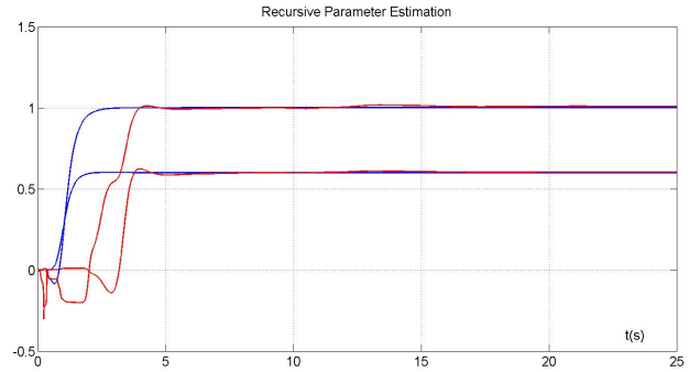
Fig. 5. Recursive parameters estimation of eq.(73) in noise free (blue lines) and noisy context (red lines)
