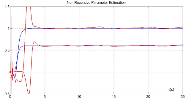
Fig. 4. Non recursive parameters estimation of eq.(73) in noise free (blue lines) and noisy context (red lines)
