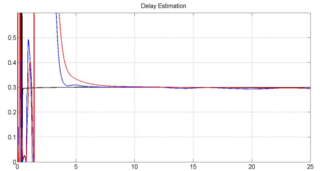
Fig. 6. Estimated delay (73) in noise free case (black line), noisy context with Procruste problem approach (eq. (69), blue line), and noisy context with updated estimation (eq. (71), red line)
