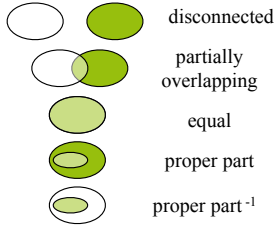
(b) relations in RCC-5
