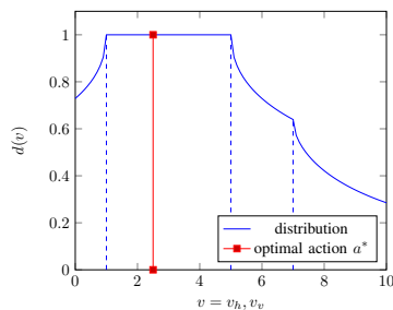
Fig. 4. Updating the representation of a distribution based on sampled actions and qualitative inference leads to a concentration around the desired but unknown action a^* after evaluating actions a = 5, 1 , and 7 .
