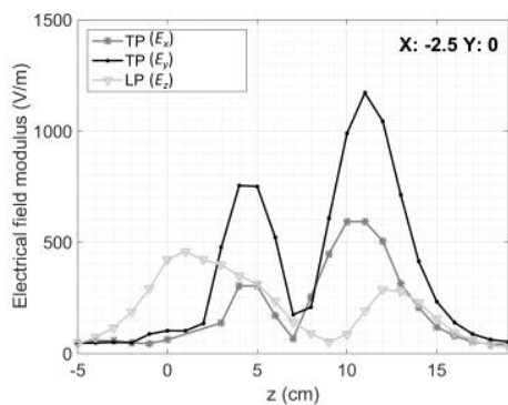
Fig 3. The three components of the E -field were measured using a transverse probe (TP) that measures the x and y -components of the E -field and a longitudinal probe (LP) that measures the z -component of the E -field. The probe was placed at X=-2.5\text{cm} and Y=0\text{cm} and moved with a 1 \text{ cm} step along the z -axis. For the three curves, two high-concentrations located at Z=5\text{cm} and Z=11\text{cm} were found and the minimum was detected at Z=8\text{cm} . The distance between the two peaks is 60 \text{ mm} which corresponds to the locations of the capacitors at distal and proximal sides of the birdcage.
