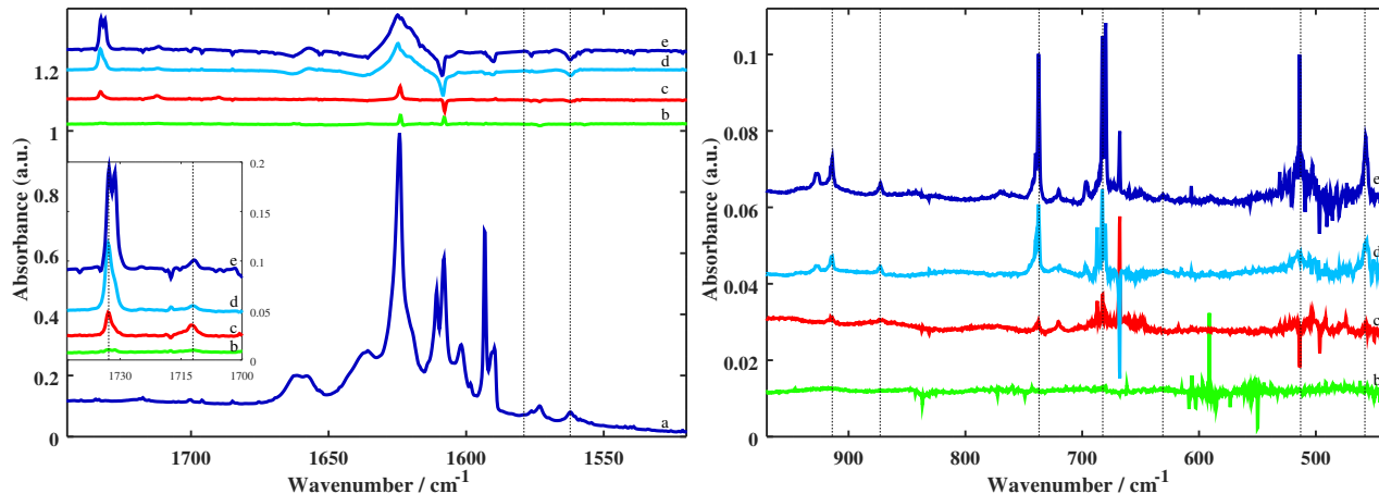
Figure 4: Processing of Fe:H 2 O:Ar matrices with UV radiation ( \lambda < 235 nm), presented in the spectral regions 1745 - 1520 \text{cm}^{-1} (left hand panel) and 970 - 400 \text{cm}^{-1} (right hand panel). In the left hand panel, spectrum a is an unprocessed Fe:H 2 O:Ar matrix (spectrum e in Fig 1), presented for comparison to the processed spectra. The spectra b–e are presented as difference spectra (irradiated minus non-irradiated samples) for increasing concentrations of H 2 O. Dotted lines represent the position of Fe:H 2 O and Fe 2 :H 2 O complexes ( 1562 and 1579 \text{cm}^{-1} ), which decrease upon irradiation. The inset presents a zoom of the 1700 – 1740 \text{cm}^{-1} region, where, upon irradiation, new bands are formed at 1733 and 1712 \text{cm}^{-1} . These are attributed to the insertion of Fe and Fe 2 into H 2 O, as has previously been reported in the literature. In the right hand panel, four spectra (traces b–e) are presented. These spectra, corresponding to the difference spectra of the four Fe:H 2 O:Ar matrices after processing with UV radiation, have the same labels as those in the left hand panel and in Figure 1. Various photoproduct absorption bands appear upon irradiation, and their attributions are detailed in Table 1 and in the text.
