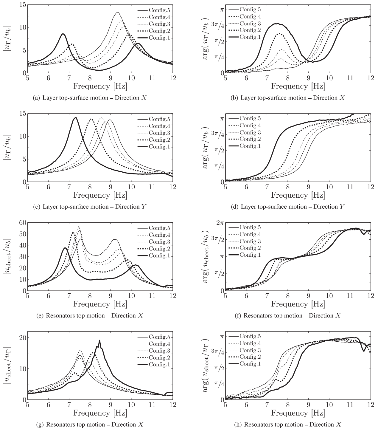
Figure 16. Experimental transfer functions for the city-configurations 1 to 5 with 37, 19, 9, 5 and 1 resonators respectively: (a) amplitude and (b) phase of the surface displacement u_r in the resonant direction X , normalized by table displacement u_b in that direction; (c) amplitude and (d) phase of the surface displacement u_r in the non-resonant direction Y , normalized by table displacement u_b in that direction; (e) amplitude and (f) phase of the displacement u_{\text{sheet}} at the top of the resonator in the resonant direction X , normalized by table displacement u_b in that direction; (g) amplitude and (h) phase of the displacement u_{\text{sheet}} at the top of the resonator in the resonant direction X , normalized by surface displacement u_r in that direction. Experimental data from central accelerometer 1 on the foam block and central resonator A.
