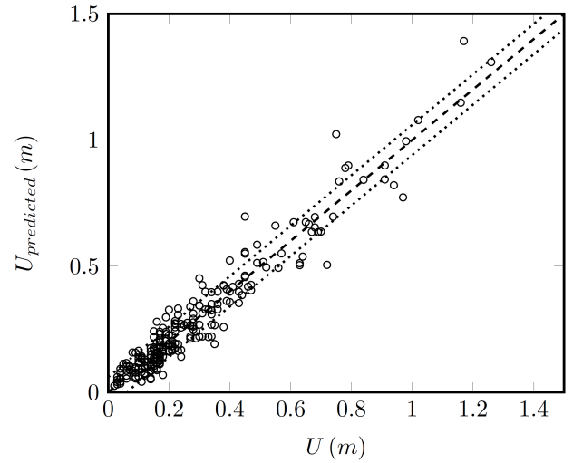
Figure 11: Newmark displacements predicted by the simplified method (Eq. 6) versus Newmark displacement calculated by the decoupled approach (circles). The dotted line represents the displacement values \pm the standard deviation \sigma .
