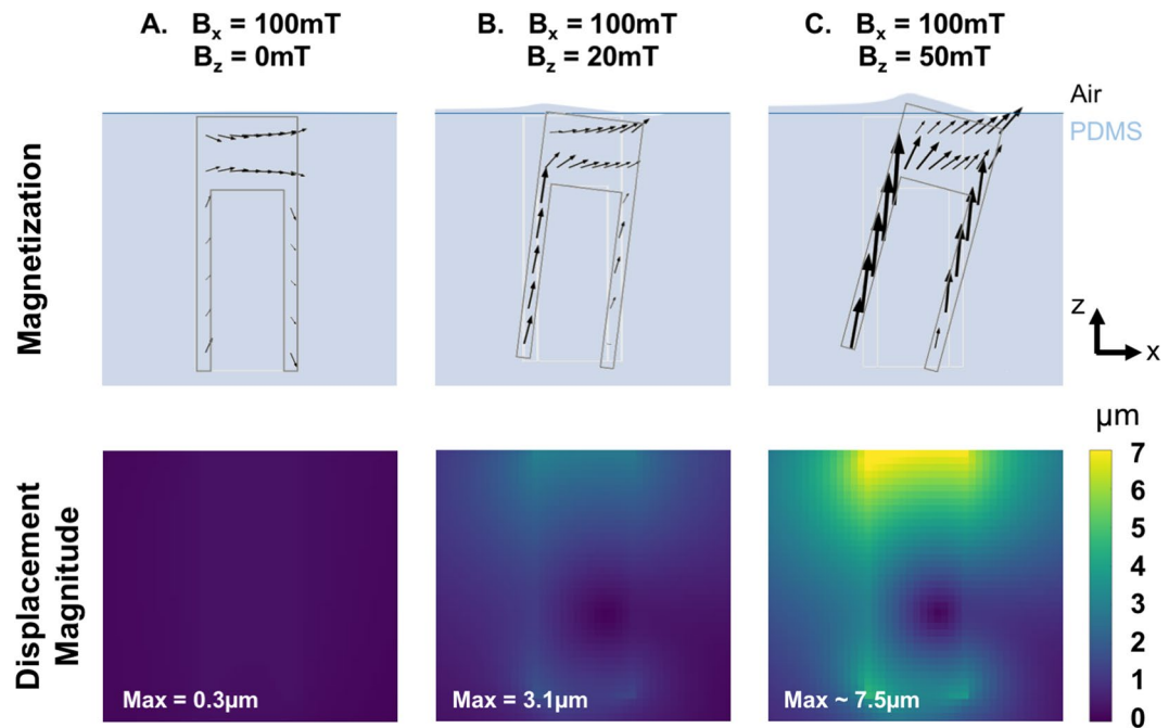
Figure 3. Contribution of B_z . The magnetization of the iron pillar induced by a purely horizontal magnetic field (A), a magnetic field with a slight (B) or large (C) vertical component B_z and the subsequent magnitude of displacement in the substrate have been predicted with the magneto-mechanical model. In each case, the undeformed positions of the PDMS free surface and the pillar are represented by blue and light grey lines, respectively.
