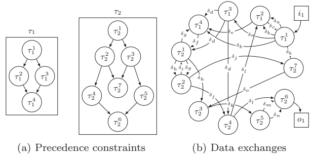
Figure 3: Example of sub-tasks dependencies.
