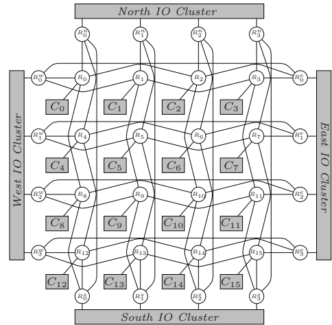
Figure 2: MPPA ® -256 architecture overview
