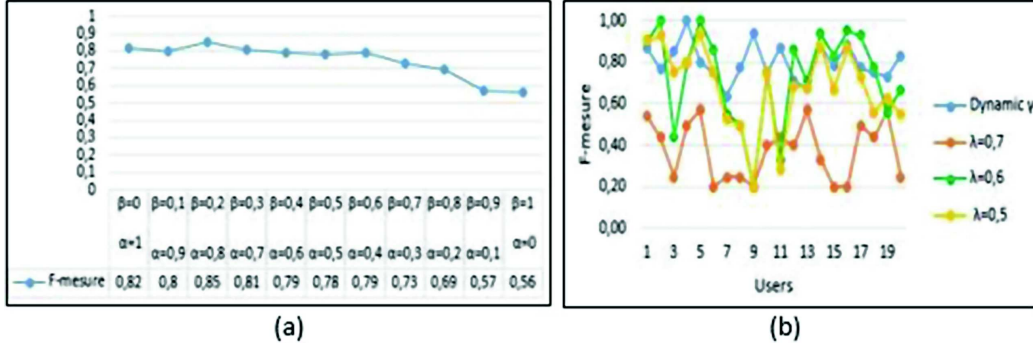
Fig. 3. (a)–Obtained results of F-measure with variation of \alpha and \beta parameters, and (b)–Obtained results of F-measure with variation of static threshold ( \lambda = 0, 5, 0, 6 and 0,7 ) compared to the dynamic threshold \gamma
