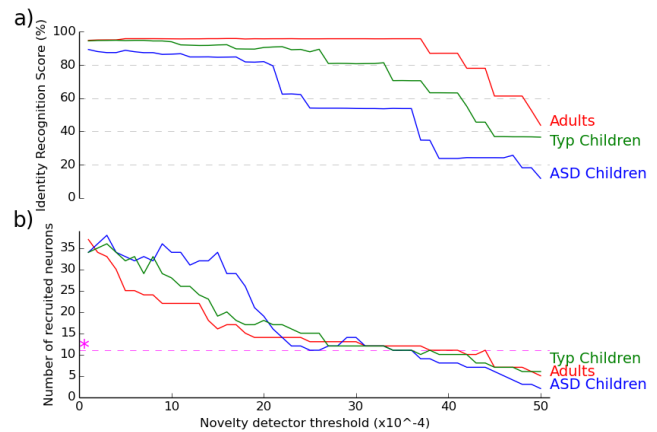
Fig. 7. Correspondence through variation of the novelty detection threshold between a) the identity recognition score for each group and b) The number of recruited neurons by the IR group of neurons to code 11 partners for each group. *Represents the minimum number of neurons possible for the identity recognition task. Less than 11 neurons for the 11 partners means the system makes a confusion between some partners
