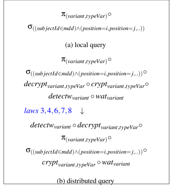
Figure 9: Query for genetic case data recovery
