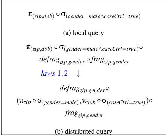
Figure 8: Query for demographic case data recovery
