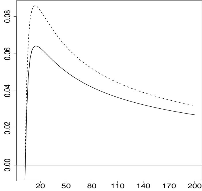
Figure 3: Extrapolation error in \text{DA}_3(\text{Gumbel}) . Vertically: Extrapolation error \varepsilon_{\text{ET}}(p_n; \alpha_n) (solid line) and its first order approximation \frac{1}{2}\eta_n^2 K_2(\log n) (dashed line) provided by Theorem 2(iii)-(a). Horizontally: \log n . Top: log-Weibull( \beta = 3 ) distribution, bottom: lognormal( \sigma = 0.5 ) distribution.
