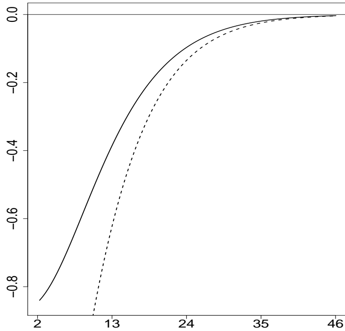
Figure 4: Extrapolation in MDA(Fréchet). Vertically: Relative extrapolation error \varepsilon_W(p_n; \alpha_n) (solid line) and its first order approximation -\frac{1}{1 - \delta_\infty} \delta(n) \log(1/\alpha_n) \eta(1/\alpha_n) (dashed line) provided by Theorem 4(i). Horizontally: \log n . Top: Burr( \rho = -1/3 ) distribution (see Section 5), bottom: Burr( \rho = -1/4 ) distribution.
