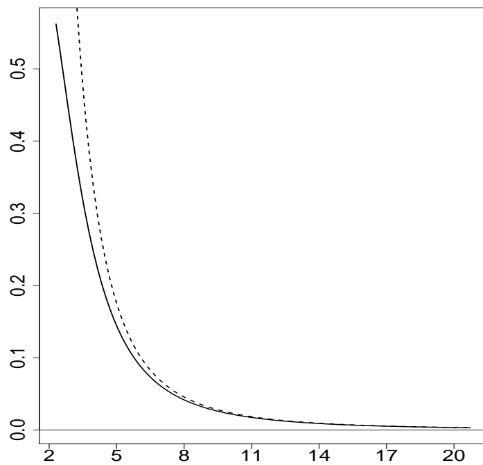
Figure 1: Extrapolation in \text{MDA}_1(\text{Gumbel}) . Vertically: Relative extrapolation error \varepsilon_{\text{ET}}(p_n; \alpha_n) (solid line) and its first order approximation \frac{1}{2}\delta^2(n)K_2(\log n) (dashed line) provided by Theorem 2(i)-(a). Horizontally: \log n . Top: Finite endpoint( \beta = 5 ) distribution, bottom: Gamma( a = 0.1 ) distribution.
