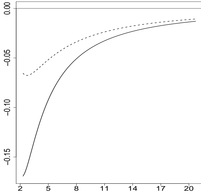
Figure 2: Extrapolation in \text{MDA}_2(\text{Gumbel}) . Vertically: Relative extrapolation error \varepsilon_{ET}(p_n; \alpha_n) (solid line) and its first order approximation \frac{\ell_1(\ell_1-1)}{2}\delta^2(n) (dashed line) provided by Theorem 2(ii)-(a). Horizontally: \log n . Top: Weibull( \beta = 5 ) distribution, bottom: Gaussian distribution.
