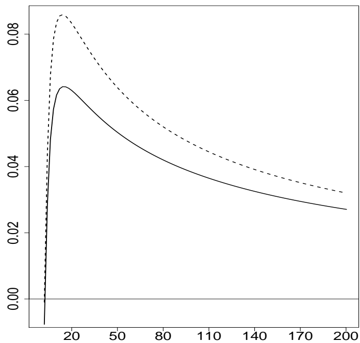
Figure 3: Extrapolation in \text{MDA}_3(\text{Gumbel}) . Vertically: Relative extrapolation error \varepsilon_{ET}(p_n; \alpha_n) (solid line) and its first order approximation \frac{1}{2}\delta^2(n)K_2(\log n) (dashed line) provided by Theorem 2(iii)-(a). Horizontally: \log n . Top: log-Weibull( \beta = 3 ) distribution, bottom: lognormal( \sigma = 0.5 ) distribution.
