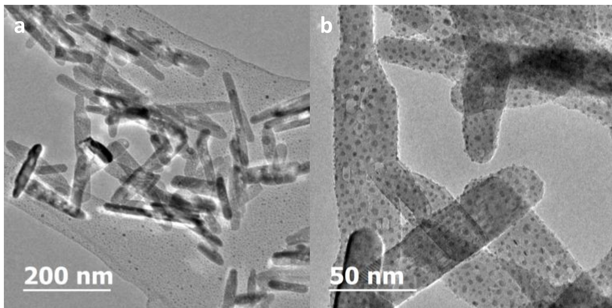
Figure 1 : (a) Low magnification TEM bright field images of rutile titania ( r -TiO 2 ) nanorods dispersed on holey carbon support film. (b) Au-Pd NPs fabricated by PLD deposited on the r -TiO 2 nanorods.
