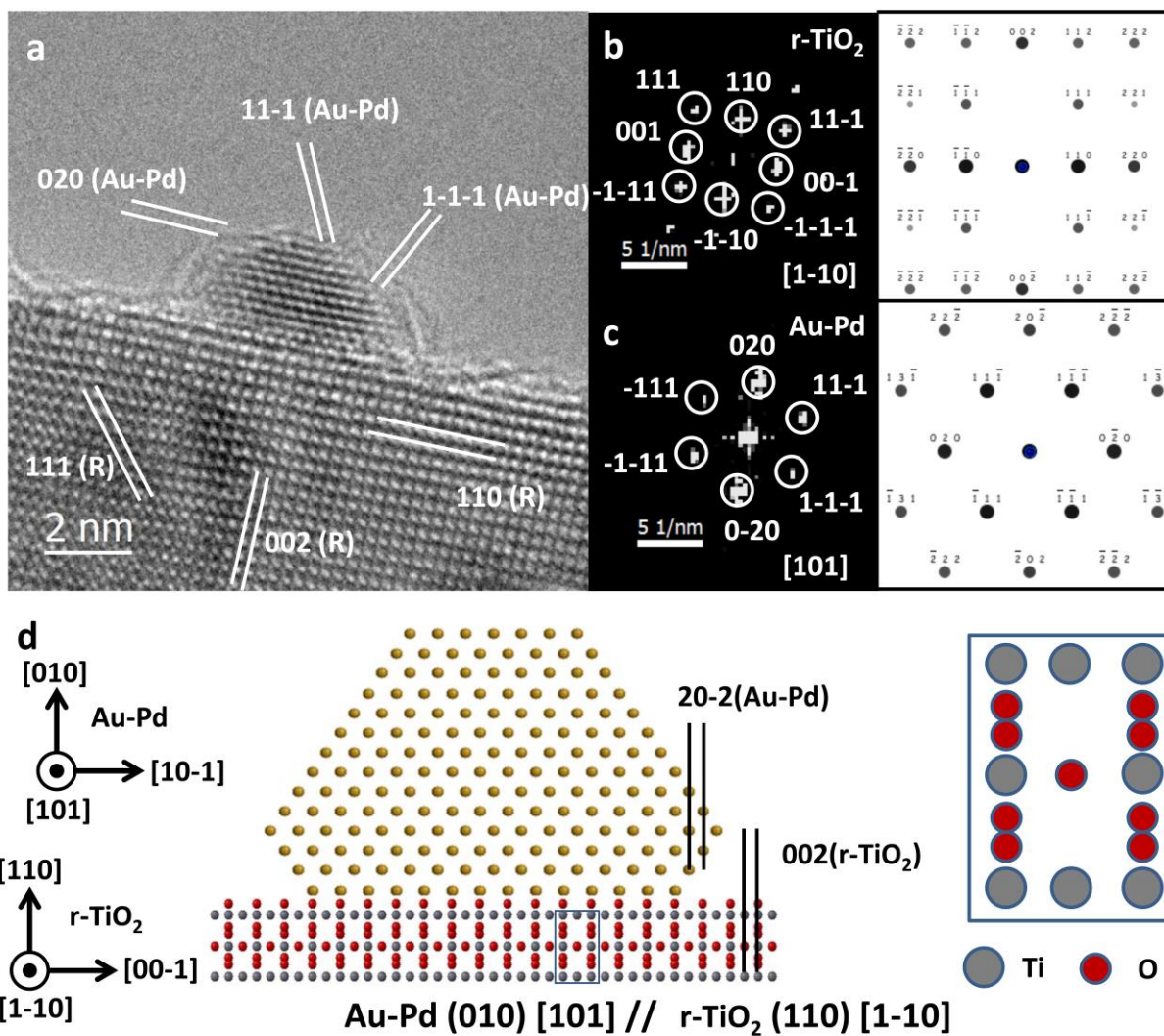
Figure 5 : Example of epitaxial relationship \text{Au-Pd} (100) [101] // r\text{-TiO}_2 (110) [1-10] : (a) HRTEM
