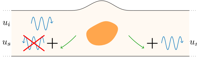
Figure 1: Schematic picture of a reflectionless mode. The propagating wave (blue) is not reflected. The backscattered field is purely evanescent (green).
