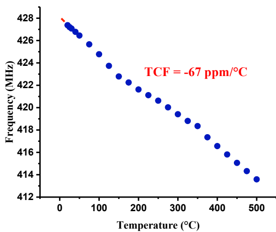
Fig. 4. Measured TCF for a 2.76 \mu\text{m} \text{ScAlN} thin film on Sapphire substrate, with \lambda = 13 \mu\text{m} .
