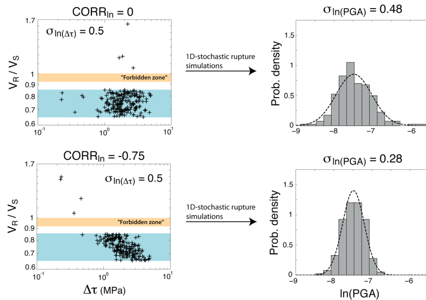
Figure 3. (left) distribution of stress drop ( \sigma_{\ln(\Delta\tau)}=0.5 ) and rupture velocity (uniform in the range [0.65V_s-0.85V_s] but assuming 2% are supershear) for different levels of correlations ( CORR_{\ln} is the coefficient of correlation between \ln(V_r) and \ln(\Delta\tau) ). (right) Resulting distribution of PGA computed using the 1-D stochastic source model.
