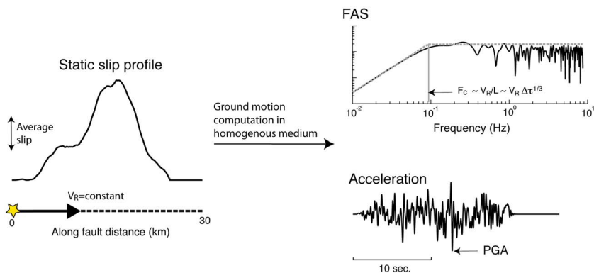
Figure 2. (a) Example of static slip distribution generated from the 1-D stochastic source model, (b) resulting Fourier acceleration spectrum, and (c) acceleration time history computed using equation (7). The example is for a rupture length L = 30 km, V_r = 2600 m/s and a source receiver azimuth of 90^\circ .
