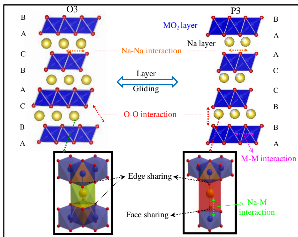
Figure. S1: Structure of O3 and P3 \text{Na}_x\text{MO}_2 ( 0 < x < 1 ), zoomed parts in the bottom showing the sodium occupation in octahedral and prismatic position of O3 and P3 phases respectively. Stability of the particular composition of \text{Na}_x\text{MO}_2 depends on the energies of the possible O-O, Na-Na, Na-M interactions mentioned in the figure.
