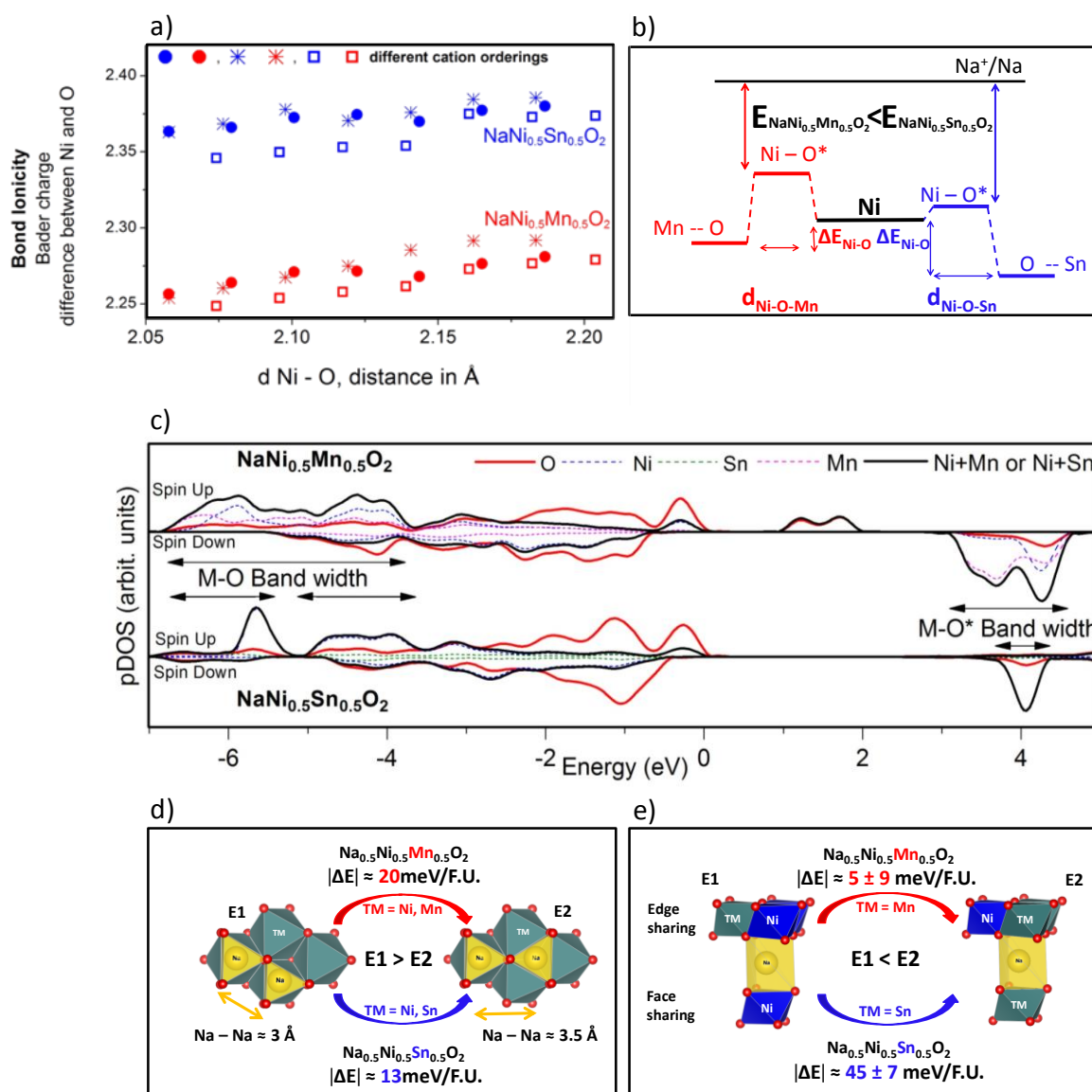
Figure 7: (a) Difference between Bader charge, obtained by DFT calculation, of Ni and O depending on the Ni – O distance in Å, tuned with the cell volume, for NaNi 0.5 Sn 0.5 O 2 in blue and NaNi 0.5 Mn 0.5 O 2 in red. Square, stars and dots stand for different Ni/Sn and
